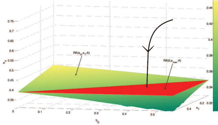
FIG. 3.5. Plot of h_A against s_T and s_Q . The green-hued surface is the sheet RK(s_Q, s_T; A) of right knees for A as a function of s_T and s_Q . The red plane is h = RK(0, s_{\max}; A) , the h value of the lowest possible right knee for A when Q has entered the silent phase. In order for A to return to the silent phase simultaneously with Q , h_A must be below the red sheet when Q enters the silent phase. We define T_A as the time it takes a trajectory starting from LK(0, 0; A) to reach the red sheet. Here, the green-hued sheet RK(s_Q, s_T; A) and the red sheet RK(0, s_{\max}; A) were generated numerically for a particular choice of the added cell A . For the added cell A , the parameters are as in Table A.1, except g_{NaP} = 2, g_L = 2 . The black trajectory, on the other hand, is fictive and included for illustrative purposes.
