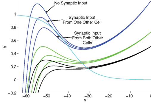
FIG. 2.3. Various levels of synaptic input to sample instances of the reduced model. The blue, green and black nullclines represent respectively a quiescent, a bursting, and a tonic cell under various levels of synaptic input. The key feature is that synaptic input from another cell lowers both the left and the right knee of the receiving cell. In this way, a quiescent cell can become bursting, and a bursting cell can become tonic.
