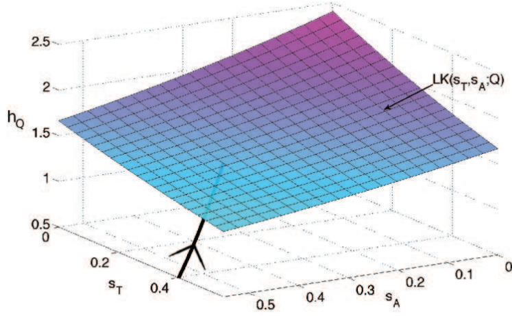
FIG. 3.3. Plot of h_Q against s_T and s_A . The multicolored surface is the sheet of Q 's left knees as a function of s_T and s_A . The black curve is the h_Q coordinate of the Q subsystem under the flow G_{LRR}(h_Q, h_A, h_T) . The trajectory evolves towards the sheet as s_T and s_A experience some decay. When trajectory reaches the sheet LK(s_T, s_A) , Q enters the active phase. From initial conditions h_Q, h_A, h_T , the time it takes the trajectory to reach the sheet is \tau_{\frac{2}{3}}(h_Q, h_T, h_A) . In this figure, the sheet of left knees LK(s_T, s_A; Q) for the quiescent cell was generated numerically, while the black trajectory is included for illustrative purposes only. For the quiescent cell Q , the parameters are as in Table A.1, except g_{NaP} = 2, g_L = 4 .
