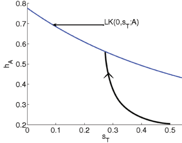
FIG. 3.1. Plot of h_A against s_T . The blue curve is the curve of the left knees of the v_A -nullcline as a function of s_T . When the black trajectory reaches the curve of left knees, the added cell A will jump up to the active phase. The time it takes to reach the curve of left knees is \tau_1^1(h_Q, h_A, h_T) for initial conditions h_Q, h_A, h_T \in W . In this figure, the blue curve LK(0, s_T; A) was generated numerically for one particular added cell A , while the black trajectory is a schematic included for illustrative purposes. For the added cell A , all parameters are as in Table A.1, except g_{NaP} = 2 , g_L = 2 .
