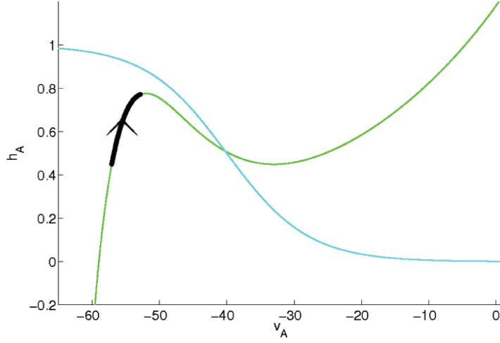
FIG. 3.2. Plot of h_A against v_A . The green curve is the v_A -nullcline, while the light blue curve is the h_A nullcline. In the worst case, shown here, the trajectory starts as high as possible, namely at RK(0, 0; A) , and continues to the left knee LK(0, 0; A) . This evolution takes time \tau_{\frac{1}{3}}^* . In this figure, the light blue and green nullclines were generated numerically for a particular choice of the added cell A , while the black trajectory is fictive and included for illustrative purposes. For the added cell A , the parameters are as in Table A.1, except g_{NaP} = 2, g_L = 2 .
