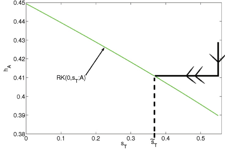
FIG. 3.4. Plot of h_A against s_T . The green curve is the curve of right knees of A as a function of s_T . The trajectory begins at LK(0, s_{max}) and has maximum velocity while s_T = s_{max} . The point with the largest value at which A can enter the silent phase is RK(0, \tilde{s}_T; A) . \tau_{\tilde{s}}^* is defined such that if s_T suddenly dropped to s_T = \tilde{s}_T after time \tau_{\tilde{s}}^* , then the trajectory of A would exactly hit the curve of knees at RK(0, \tilde{s}_T; A) . In this figure, the green curve RK(0, s_T; A) of right knees was generated numerically for a particular choice of the added cell A . For the added cell A , the parameters are as in Table A.1, except g_{NaP} = 2, g_L = 2 . The black trajectory is an illustration of the worst-case trajectory and may not be realized.
