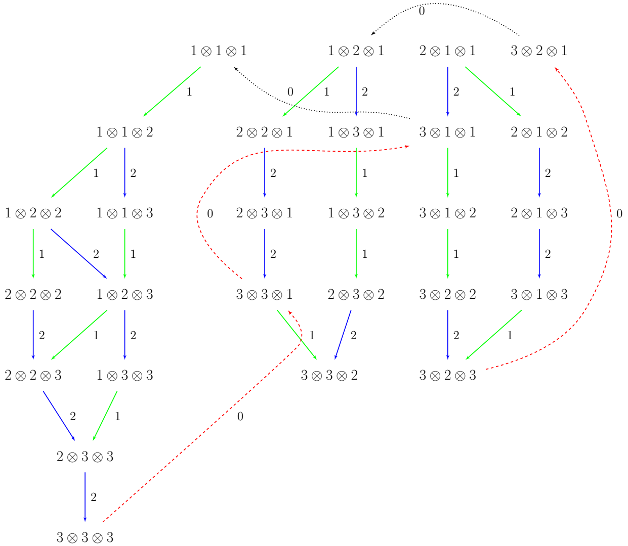
A combinatorial model for the representation of \mathfrak{sl}_3 and the quantum affine algebra U_q(\widehat{\mathfrak{sl}}_3) on V^{\otimes 3} , for V = \text{span}(e_1, e_2, e_3) .
