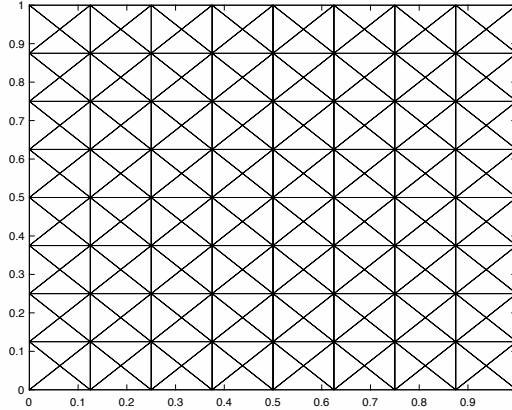
FIG. 6.1. Computational mesh for \Omega corresponding to h = 1/8 .
