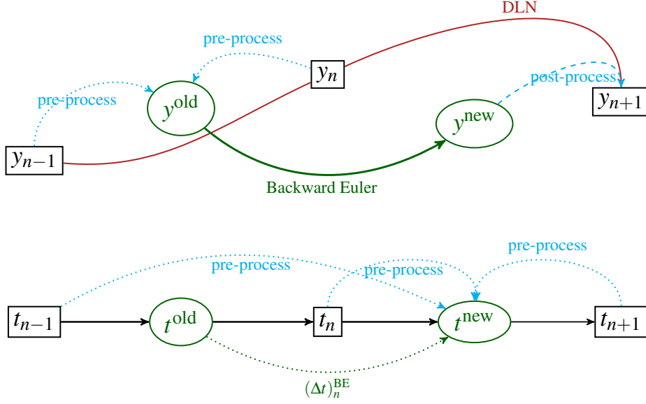
FIG. 2.1. Refactorization of the (DLN) method as a pre- and post-processed (BE) method
