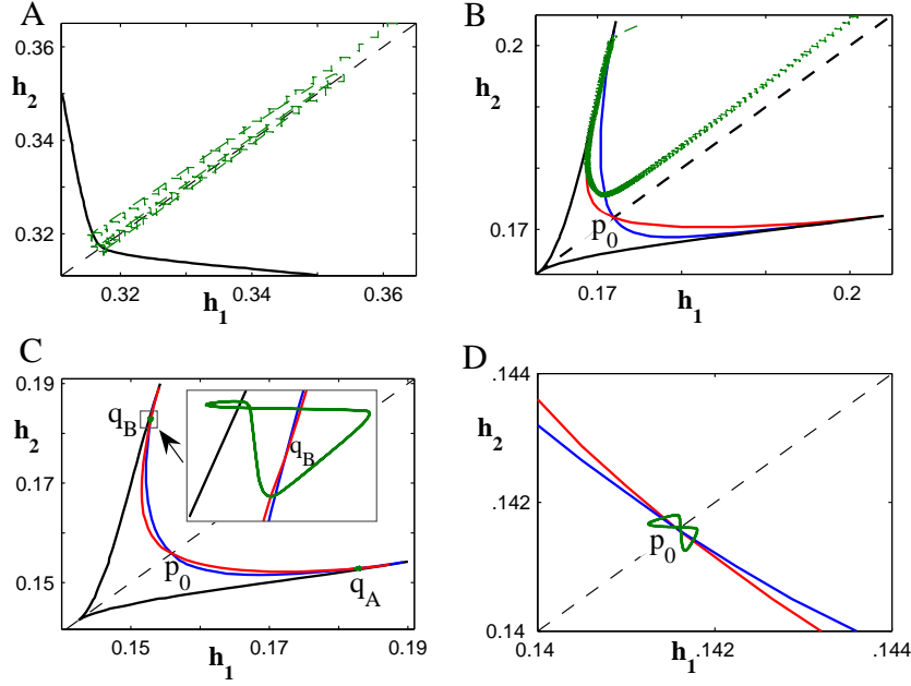
Figure 11: Averaged phase planes, corresponding to (6), with superimposed trajectories of (1)_i - (4)_i , for g_{syn-e} = 3 . Throughout this figure, the jump-down curve \mathcal{B} is solid black, the nullclines \mathcal{A}_1, \mathcal{A}_2 are red and blue, respectively, the symmetry axis \mathcal{L} is dashed black, and trajectories are green. A) For g_{tonic-e} = .57 , \dot{h}_1, \dot{h}_2 are negative everywhere in the oscillatory region \mathcal{O} . Thus, every solution of the averaged equations leaves the oscillatory region \mathcal{O} through \mathcal{B} and the system exhibits symmetric bursting. B) For g_{tonic-e} = .83 , there is an unstable fixed point p_0 in \mathcal{O} where the averaged nullclines intersect. The system exhibits asymmetric bursting. C) For g_{tonic-e} = .87 , the averaged nullclines intersect at three fixed points in \mathcal{O} , namely p_0 , which is still unstable, and q_A, q_B , which are stable. The system exhibits asymmetric tonic spiking. An asymmetric tonic spiking solution is shown in green; similar solutions exist near q_A . D) For g_{tonic-e} = .91 , p_0 is a stable fixed point and the system exhibits symmetric spiking. Here \mathcal{B} is not visible since it lies at smaller (h_1, h_2) values than those shown in this plot.
