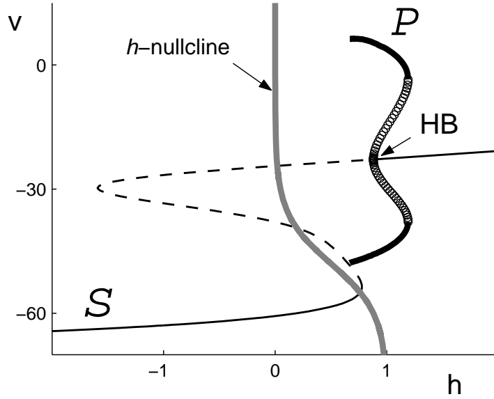
Figure 1: The bifurcation diagram for the fast subsystem (1),(3) with (g_{tonic-e}, g_{syn-e}) = (0.2, 0) , projected into (h, v) -space, along with the h -nullcline. The solid (dashed) black curve is the curve \mathcal{S} of stable (unstable) critical points of (1),(3) with h fixed at the levels indicated on the abscissa. A family of unstable periodic orbits, with maxima and minima labeled by open circles, emanates from \mathcal{S} in a Hopf bifurcation at the point marked HB. This family coalesces with the family of stable periodic orbits \mathcal{P} , with maxima and minima labeled by dark, thick curves, in a saddle-node bifurcation at h near 1.3. The thick grey curve shows the h -nullcline, namely h = h_\infty(v) , where h' = 0 .
