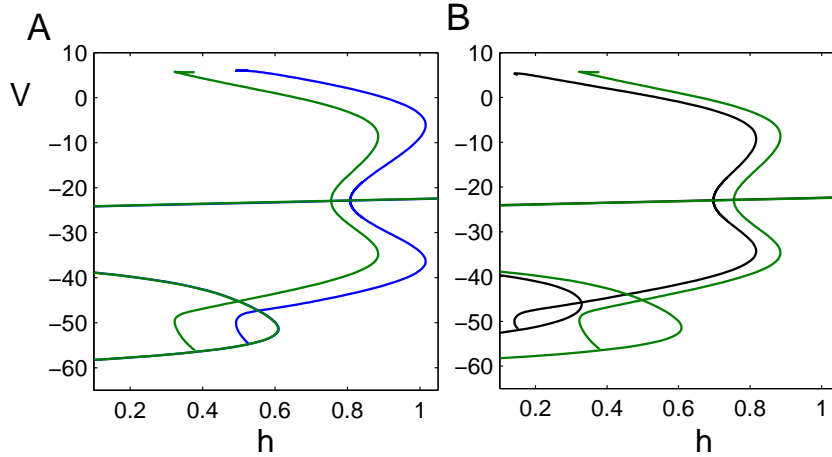
Figure 19: Changes in \mathcal{AP}_S induced by changes in g_{syn-e} and g_{tonic-e} . A) With g_{tonic-e} = 0.3 , increasing g_{syn-e} from 4 (blue) to 8 (green) moves \mathcal{AP}_S , and the corresponding Hopf point, to the left, while the lower knee of \mathcal{S} remains unchanged. B) With g_{syn-e} = 8 , increasing g_{tonic-e} from 0.3 (green) to 0.6 (black) moves both \mathcal{AP}_S and the lower knee of \mathcal{S} to the left. (Note that the red copies of \mathcal{AP}_S in both panels are identical.)
