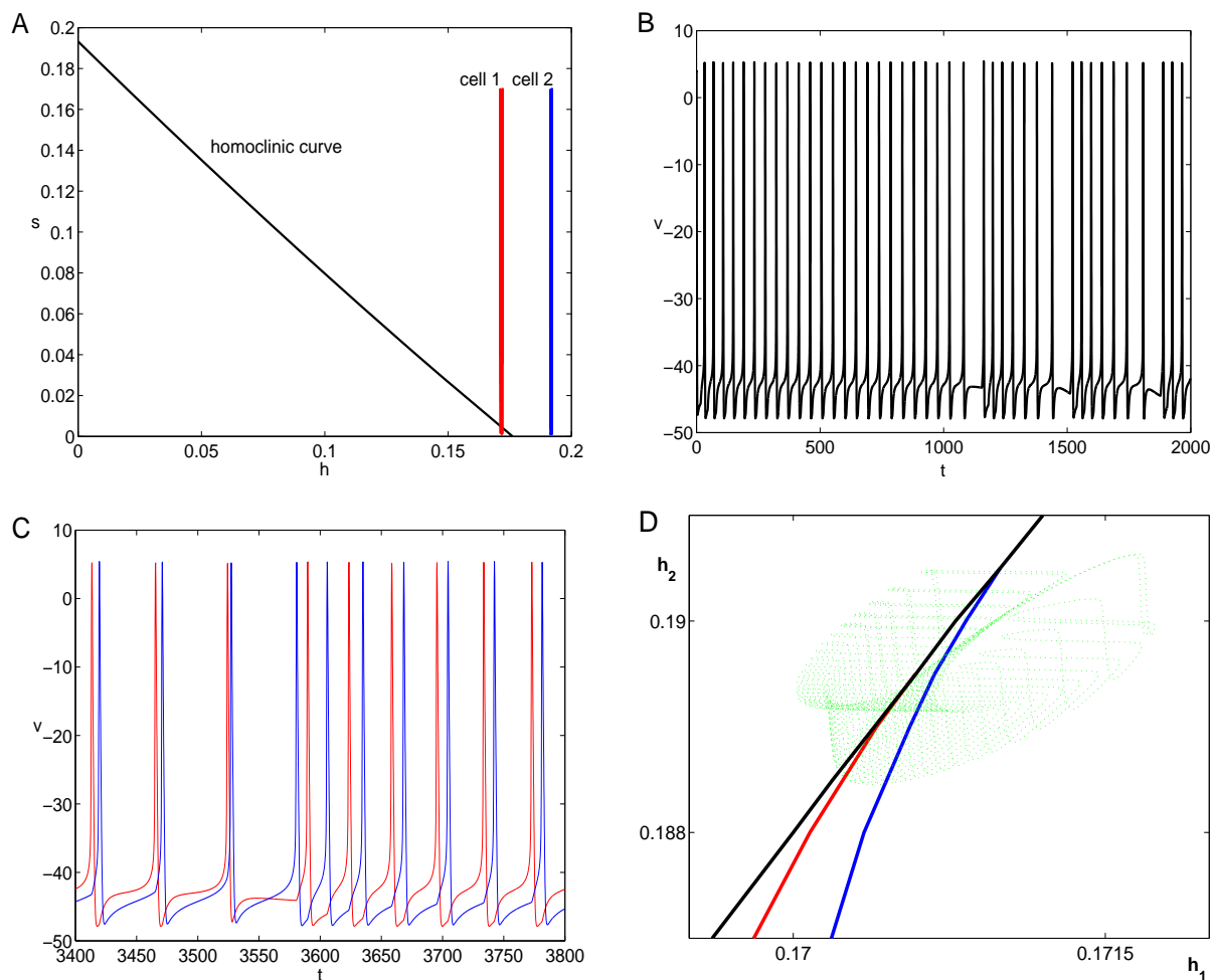
Figure 17: The sustained oscillations of one cell can rescue the oscillations another cell to which it is coupled, as shown here for g_{syn-e} = 2, g_{tonic-e} = 0.88 . A) Even when cell 1 crosses from above to below the curve of homoclinic orbits ( \mathcal{H} in the text), cell 2 continues to oscillate. The coupling from cell 2 pulls cell 1 back across \mathcal{H} , where it resumes oscillations. B) The transition across \mathcal{B} yields a switch from tonic spiking to irregular sustained oscillations in the dynamics of the fast subsystem (1)_i, (3)_i, (4)_i . Here, a crossing of \mathcal{B} was implemented by decreasing h_1 from .1693 to .1692 at time 999, with h_2 = .205 . The v time course is only shown for one cell; it was qualitatively similar for the other cell. C) The dynamics of the full system shows asymmetric bursting with short interburst intervals, with a change in burst cycle occurring when cell 2 (blue) fires two consecutive spikes. D) This asymmetric bursting solution (green) remains very close to \mathcal{B} (black) in the (h_1, h_2) plane; the red and blue curves show the nullclines \mathcal{A}_1, \mathcal{A}_2 of (6) as they terminate on \mathcal{B} .
