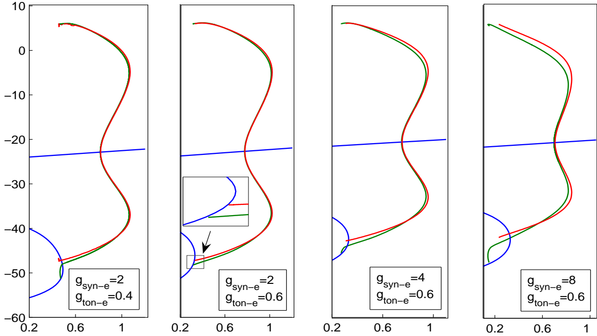
Figure 20: Changes in the anti-phase (green) and in-phase (red) periodic orbit families as g_{tonic-e} and g_{syn-e} vary. As g_{tonic-e} is increased for fixed g_{syn-e} , the anti-phase family switches from three branches, connected by two saddle-node bifurcations, to two branches, corresponding to the switch from top hat bursting to square-wave bursting. Lowering g_{syn-e} for fixed g_{tonic-e} has a similar effect.
