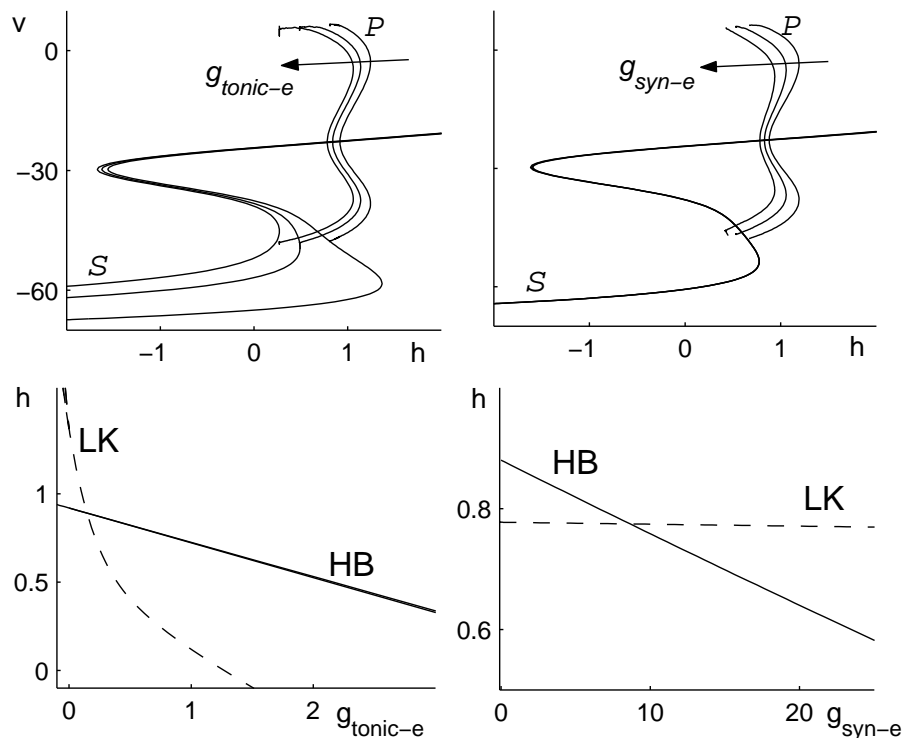
Figure 2: Dependence of the bifurcation structure of (1),(3),(4) on g_{tonic-e} and g_{syn-e} . The upper plots show curves of critical points and families of periodic orbits for varying values of g_{tonic-e} and g_{syn-e} . Left: g_{tonic-e} = 0, 0.4, 0.7, g_{syn-e} = 0 . Right: g_{tonic-e} = 0.2, g_{syn-e} = 0, 4, 8 . Larger values correspond to more leftward structures. The bottom plots show how the positions of the lower knee (LK) and Hopf bifurcation point (HB) vary with g_{tonic-e} (with g_{syn-e} = 0 ) and g_{syn-e} (with g_{tonic-e} = 0.2 ), respectively. Note that the lower knee, and indeed the entire curve of critical points, are approximately invariant under changes in g_{syn-e} .
