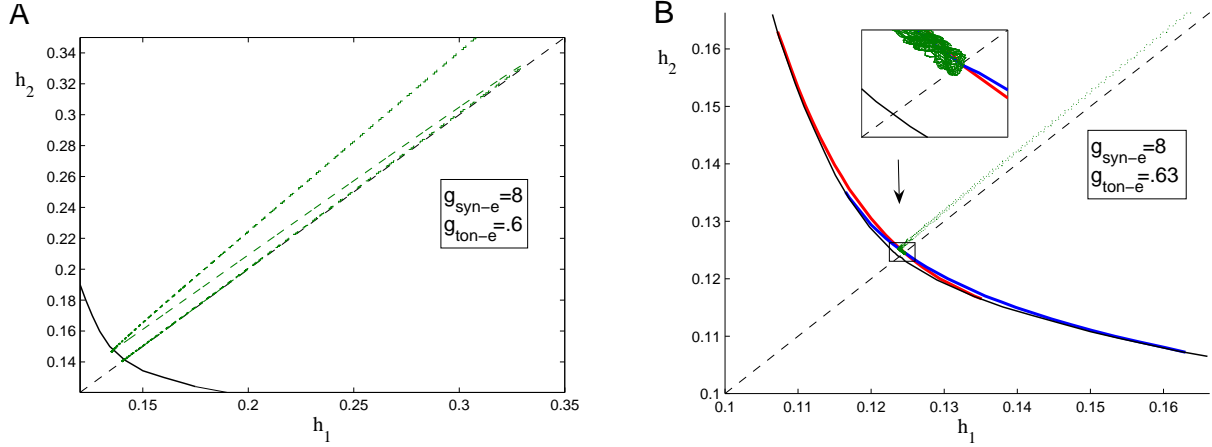
Figure 14: Averaged phase planes from (6), with superimposed trajectories of the full system, for g_{syn-e} = 8 , corresponding to a direct transition from SB to SS. The labels here are as in Figure 11. A) Symmetric bursting solution for g_{tonic-e} = .6 . The green trajectory shown travels first from the upper right part of the region to the lower left, where it hits the black boundary curve \mathcal{B} . At this point, the cells enter the silent phase and h_1, h_2 both increase. Correspondingly, the trajectory here moves back from lower left to upper right, although the cells are not spiking and the dynamics of (6) are irrelevant. The jump up to the active phase for the next burst cycle corresponds to the trajectory turning around and heading back toward \mathcal{B} . Note that h_1 and h_2 become closer during the silent phase and jump-up, such that the trajectory subsequently travels close to \mathcal{L} (black dashed line). B) Symmetric spiking solution for g_{tonic-e} = .63 . The red and blue curves are the nullclines \mathcal{A}_1 and \mathcal{A}_2 , respectively, of (6). The inset shows how the sample trajectory shown approaches the fixed point p_0 where \mathcal{A}_1 \cap \mathcal{A}_2 occurs.
