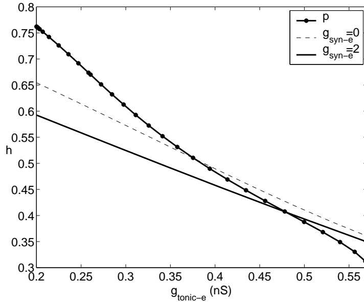
Figure 4: The curve of fixed points p of (1)-(4), together with the curves of homoclinic points \mathcal{P} \cap \mathcal{S} of the fast subsystem (1),(3),(4) for g_{syn-e} = 0 and g_{syn-e} = 2 , as a function of g_{tonic-e} . The intersections of these curves yield the values of g_{tonic-e} at which the transition from bursting to tonic spiking is predicted to occur, based on a fast/slow decomposition of the single self-coupled cell. Note that although p switches from the lower branch of \mathcal{S} to the middle branch at g_{tonic-e} \approx 0.26 , the h -value of p is a monotonically decreasing function of g_{tonic-e} , because all of \mathcal{S} moves toward smaller h values as g_{tonic-e} increases.
