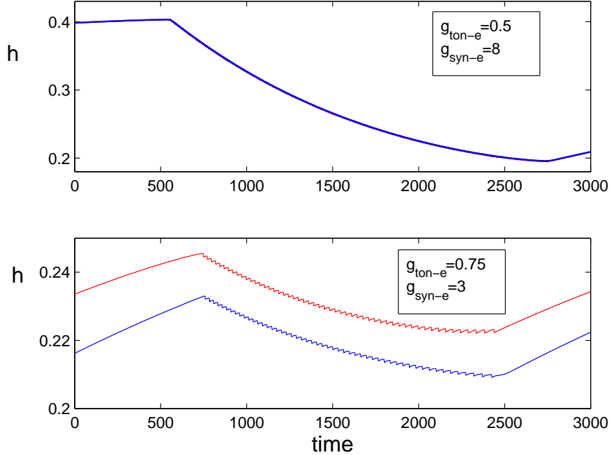
Figure 7: Plots of h_1 (red) and h_2 (blue) as functions of time during a single burst cycle. If g_{\text{syn-e}} is large (top), then h_1 \approx h_2 , while for moderate or low values of g_{\text{syn-e}} (bottom), we cannot assume that h_1 \approx h_2 .
