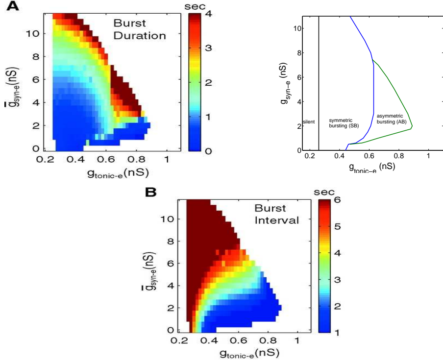
Figure 18: Simulated burst durations and (inter)burst intervals from Butera et al. [2]. A) The color-coded plot shows how burst duration in a pair of coupled pre-BötC cells changes with g_{tonic-e} and g_{syn-e} . The transition curves that we have computed for the onset and offset of symmetric and asymmetric bursting, from Figure 13, are shown for comparison, illustrating in particular that the transition from symmetric to asymmetric bursting is responsible for the abrupt increase in burst duration with g_{tonic-e} . B) Interburst interval increases with g_{syn-e} and decreases with g_{tonic-e} . The color-coded plots of burst duration and interburst interval shown here appeared in [2] and are used with permission of the American Physiological Society.
