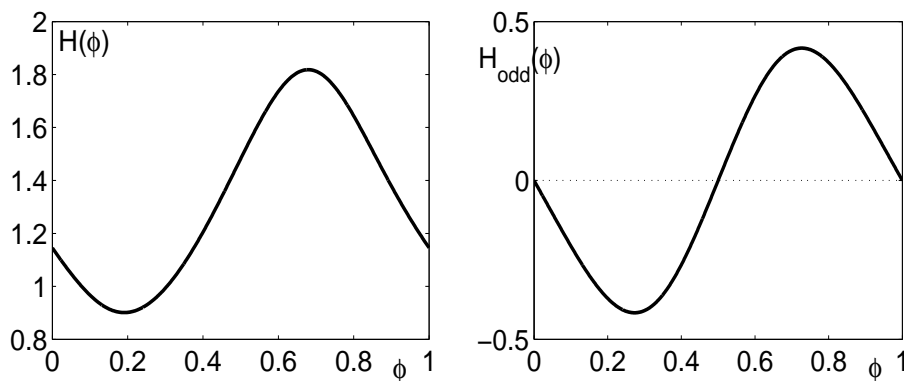
Figure 12: H -function and its odd part H_{odd} for g_{tonic-e} = 1.05 and g_{syn-e} = 1 . Since H_{odd}(0.5) = 0 and H'_{odd}(0.5) > 0 , the anti-phase symmetric spiking solution is predicted to be stable.
