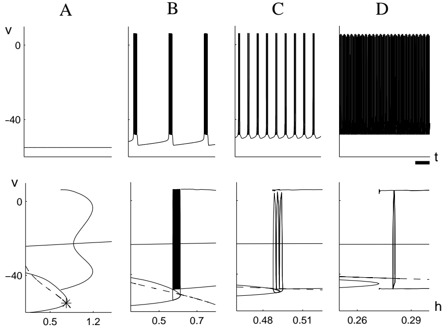
Figure 3: Voltage traces (top row) and bifurcation diagrams with superimposed trajectories (bottom row). In all panels, g_{syn-e} = 0 . The parameter g_{tonic-e} takes values 0.2 (A - quiescence; stable critical point on the lower branch of \mathcal{S} denoted by *), 0.3 (B - bursting), 0.4 (C - bursting), and 0.7 (D - tonic spiking). In the top row, the scale bar corresponds to 2 sec. Note the different h -axis scales in each panel in the bottom row.
